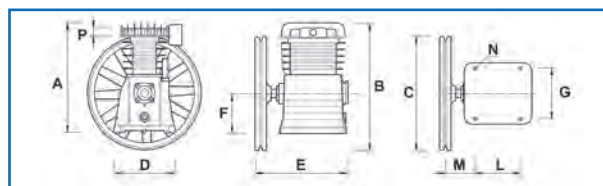
Single stage belt driven compressor pumps
