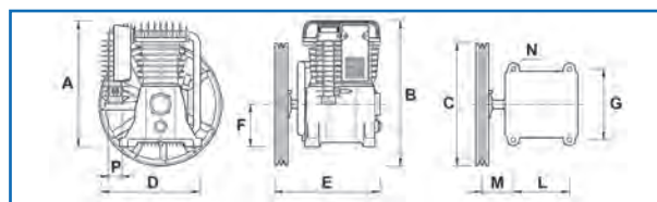
Two stages belt driven compressor pumps
